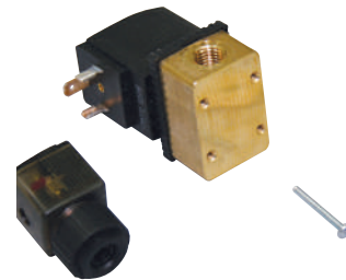
3/2 NORMALLY OPEN SOLENOID, 110V COIL WITH DIN PLUG Part # 90-141-24-PP
