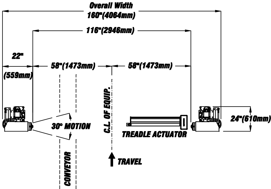
PLAN VIEW ELIMINATOR RW-103 (SHOWN WITH TREADLE)
