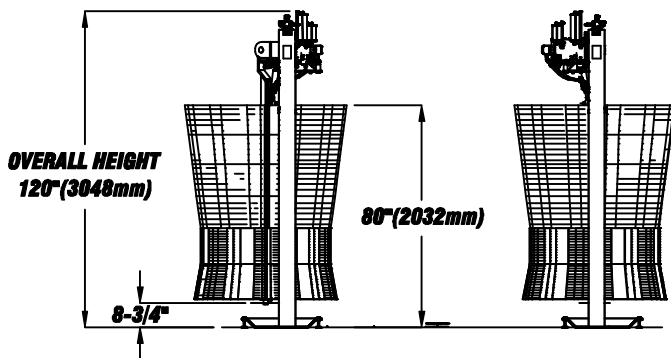
FRONT VIEW SuperFlex RS-701B Free Standing
