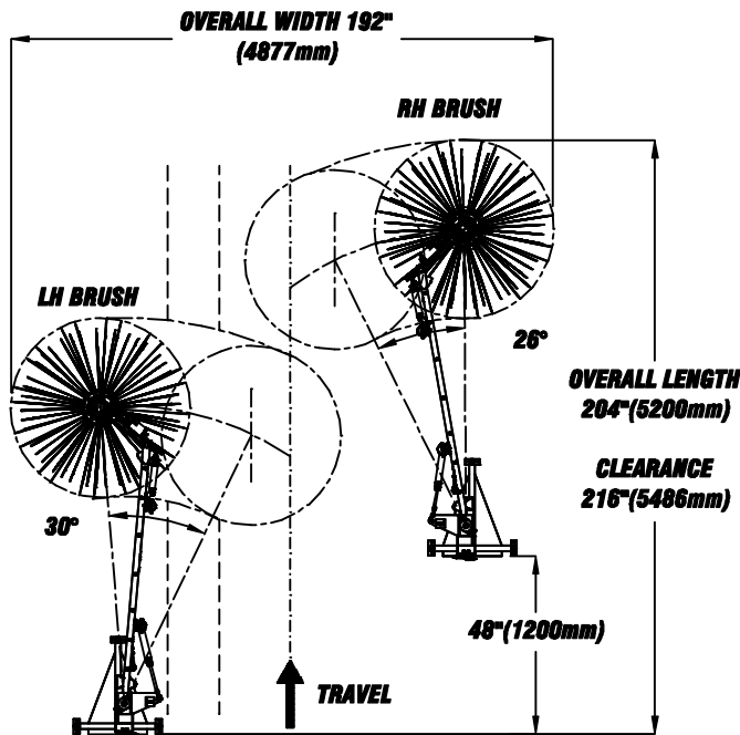
PLAN VIEW SuperFlex RS-701B Free Standing (Shown With Double Long Arm)
