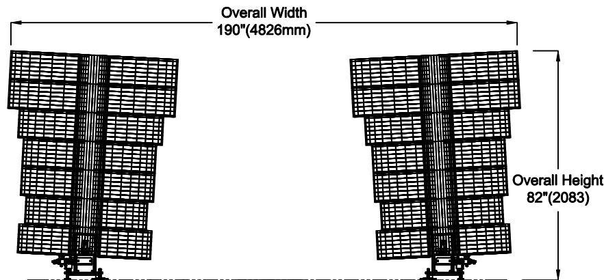
FRONT VIEW HIGH SIDE WASHER RS 301
