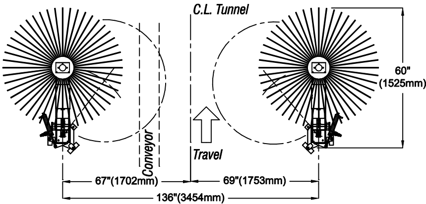
PLAN VIEW HIGH SIDE WASHER RS 301
